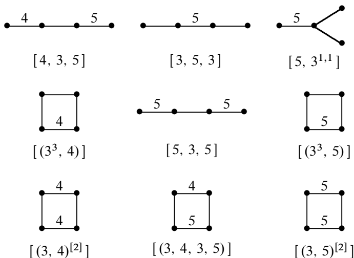
Figure 1. Cocompact hyperbolic Coxeter tetrahedral groups.
